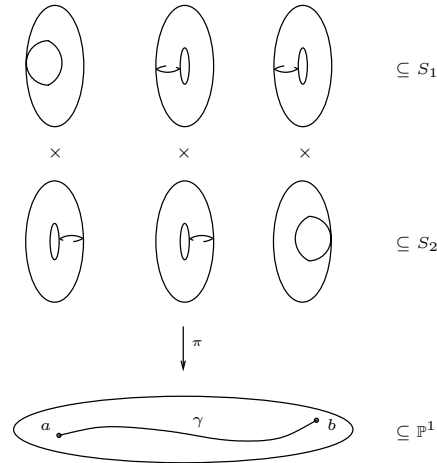
Figure 1: Fibred Lagrangian three-spheres.
